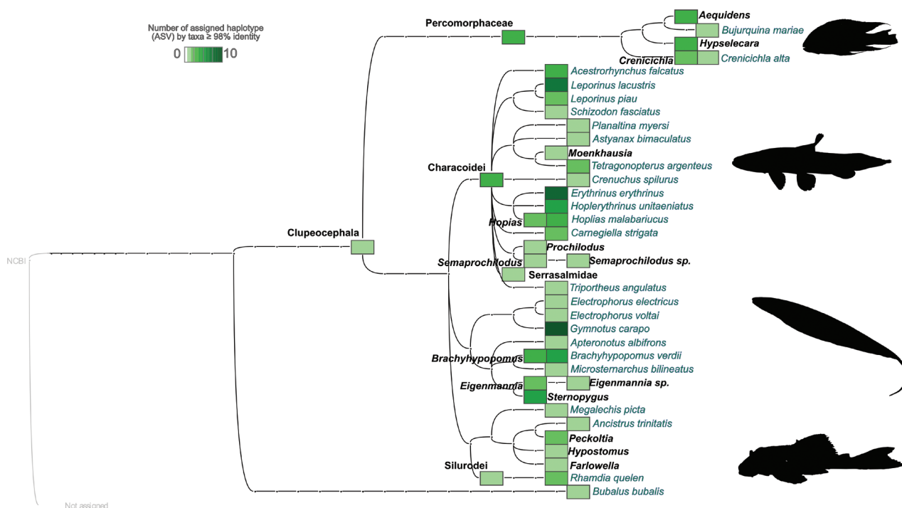
Figure 2. Taxonomic assignments using the LCA algorithm with default parameters and setting the minimum percent identity to 98.0% with MEGAN6.
