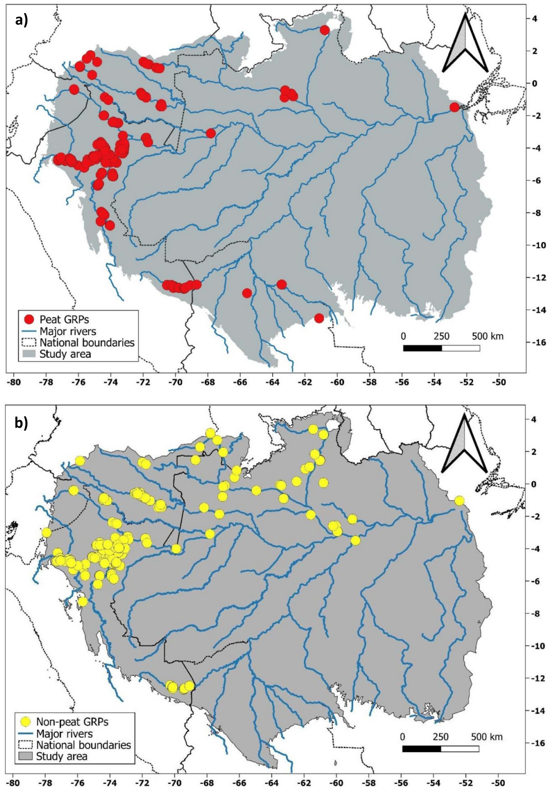
Figure 1. Distribution of (a), the peat ground reference points (GRPs) and (b), non-peat GRPs sampled for peat presence/absence, peat thickness (where present) and vegetation cover used in this study.
