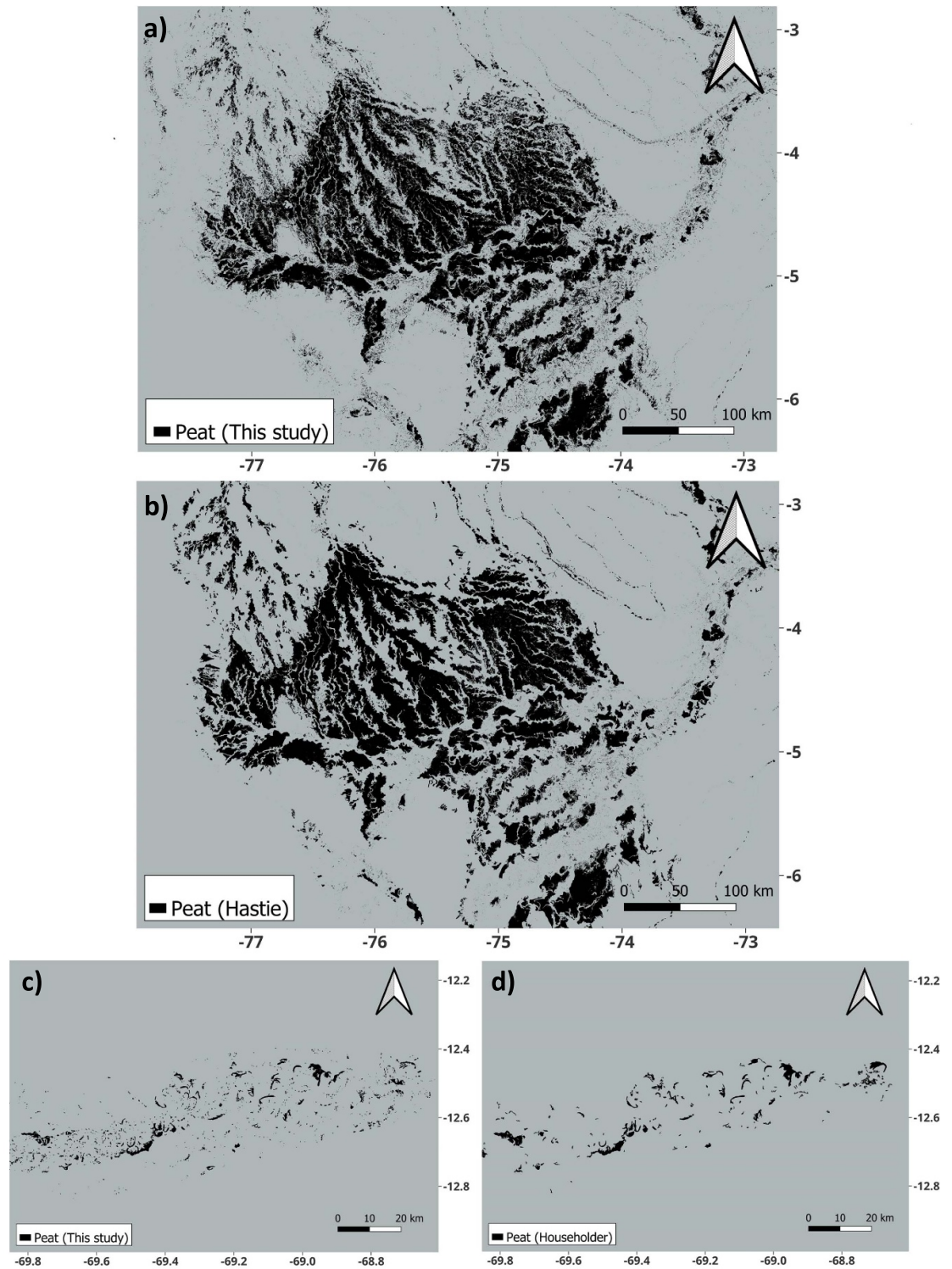
Figure 5. Predicted peat extent (a), across northern Peruvian Amazonia in this study, (b) across northern Peruvian Amazonia in Hastie et al (2022), (c), across the eastern Madre De Dios basin in this study, (d), across the eastern Madre De Dios basin in Householder et al (2012). Adapted from Hastie et al (2022), with permission from Springer Nature. Adapted from Householder et al (2012), with permission from Springer Nature.
