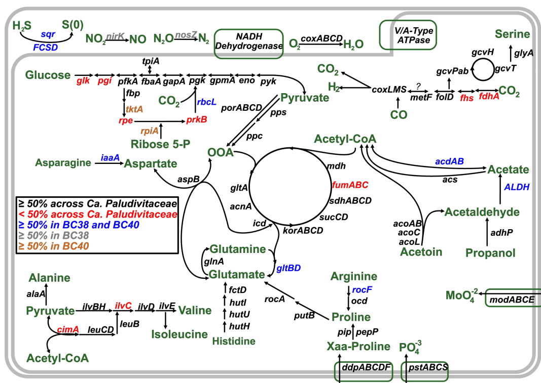
FIG 3 Proposed key (high frequency) and variable metabolic characteristics in Ca. Paludivivaceae . Gene names are color-coded by the frequency of MAGs with that gene by BC. Key intermediates and pathway outputs are displayed in green. Question mark symbol represents an unknown function. A detailed list of corresponding KEGG numbers, gene names, and presence/absence in respective MAGs are listed in File S3.
