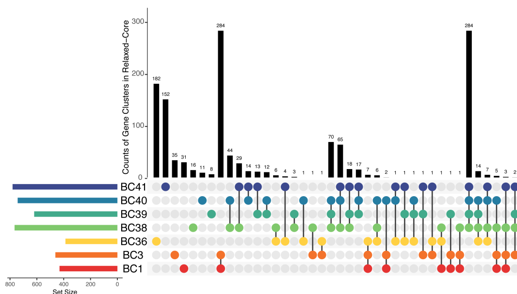
FIG 5 Meta-pangenome analysis of selected BC clades: BC1, BC3, BC36, BC38, BC39, BC40, and BC41. Upset plots (78) show the distribution (upper black columns) and overlap of gene clusters between BCs (connected circles) found within the relaxed-core of clades (indicating the size of the set of genes in lower left bars).
