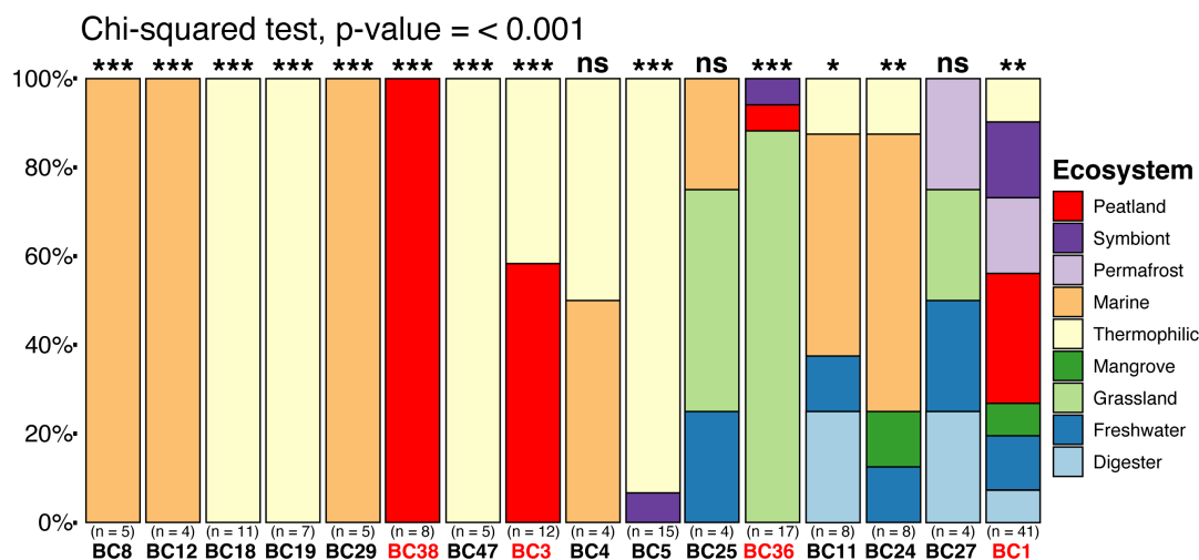
FIG 2 Mosaic plot of the frequency of MAGs recovered by ecosystems in BCs with more than four representatives. BC labels in red represent clades with PMFB MAG representatives. Asterisks above each column represent the significance level of the relationship of an ecosystem to BC. Significance scale is as follows: *** - (0,0.001), ** - (0.002,0.01), * - (0.01,0.05), ns, not significant.
