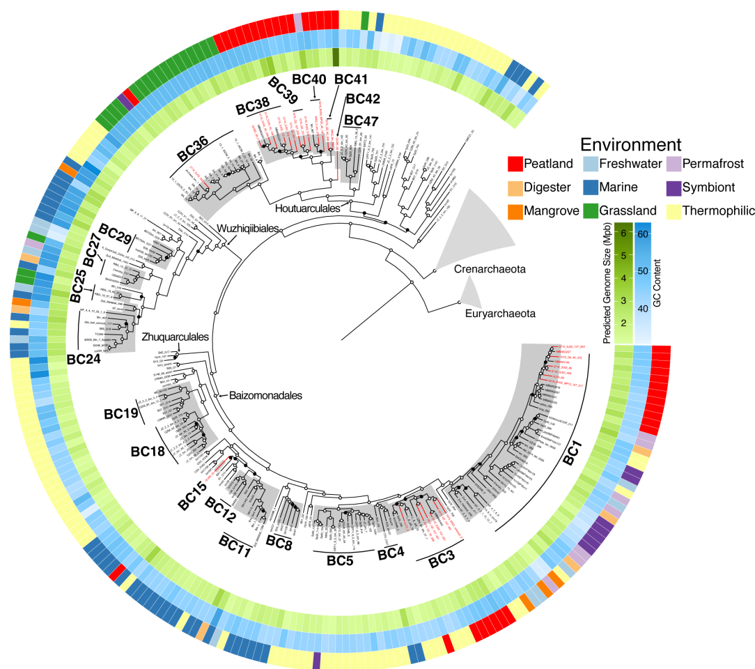
FIG 1 Maximum likelihood phylogenetic inference of 233 Bathyarchaeia MAGs constructed using 54 concatenated protein sequences. The robustness of MAG placement was assessed using 300 bootstrapping support. Bootstrap support of \geq 70\% and < 70\% (black) is represented by hollow and black circles, respectively. Clades with gray backgrounds and that are labeled represent potential genera (based on tree topology and AAI) with more than four MAGs. MAGs recovered from the PMFB are in red. Orders with representatives from the PMFB are labeled at the node. Corresponding heatmaps display the predicted genome size and GC%, for each along with the environmental source from which each MAG was recovered.
